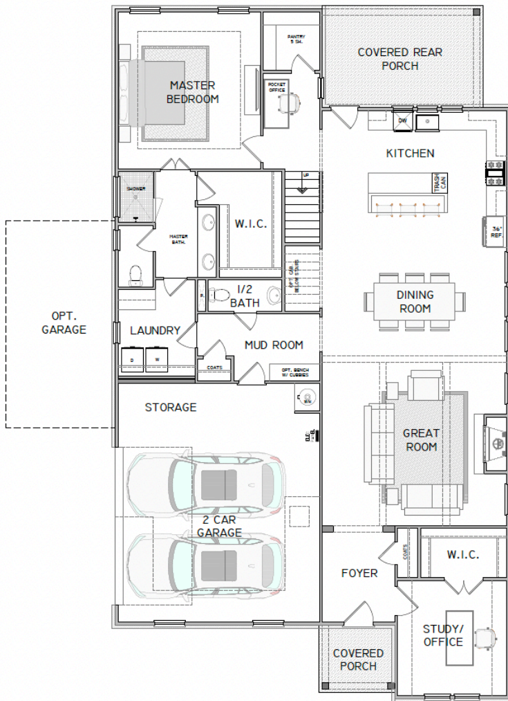
1ST FLOOR
