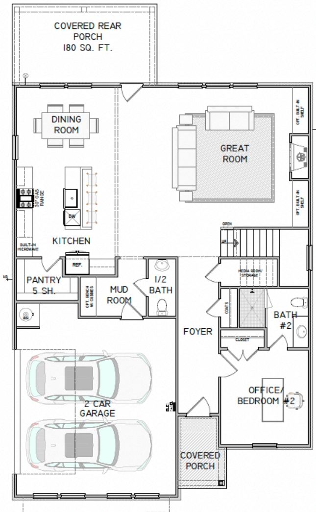
1ST FLOOR
