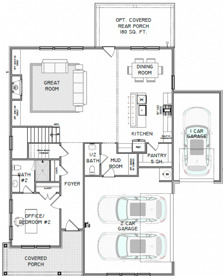
1ST FLOOR
