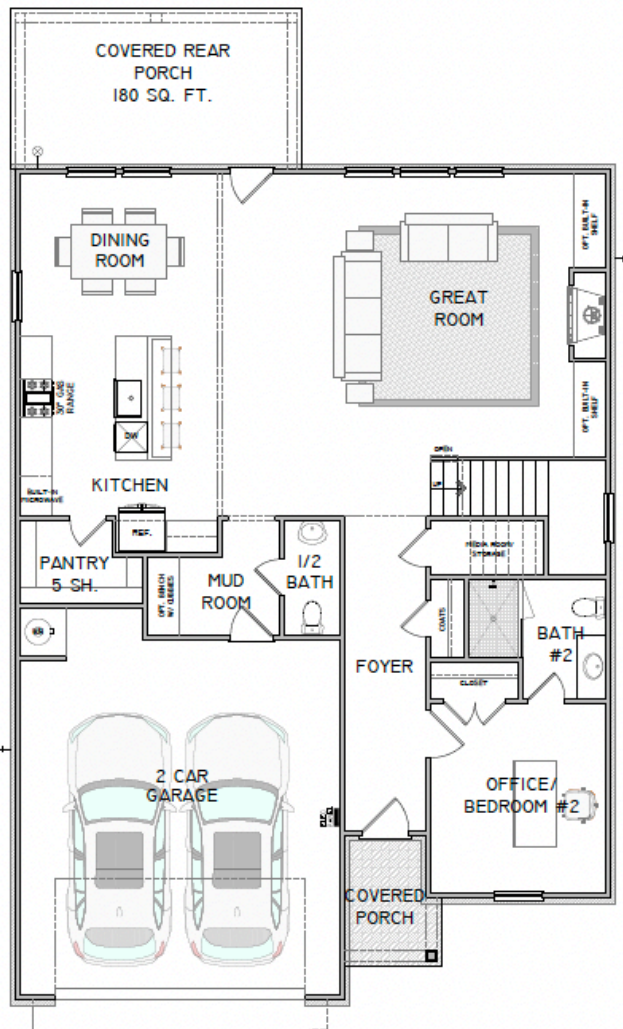
1ST FLOOR
