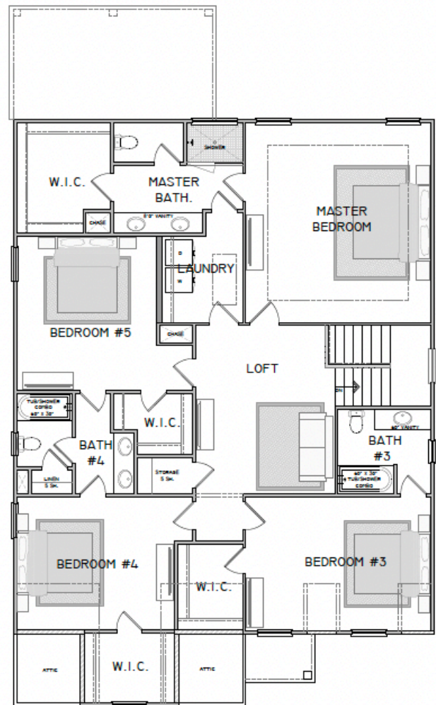
2ND FLOOR
